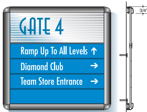
2000 Radius Series - 15"w x 15"h Anodized aluminum frame with raised cut-out graphics on perforated header panel and strips are painted with VDC letters.
