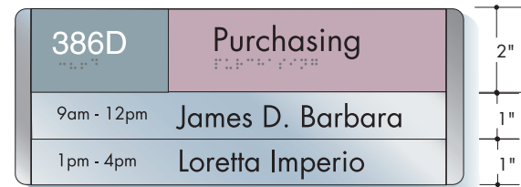
AM series 4" x 10" with (2) 1" h & (2) 2" h modules w/rounded end closure bars
