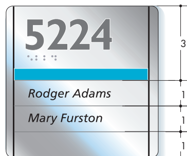
AM series 6" x 6" with /(3) 1" h copy modules & (1) 3" h ADA raised copy & braille & color accent
